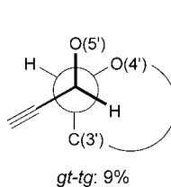
Fig. 2. Calculated population of the conformations obtained by rotation about the C(5')–C(4') bond of \beta -D-ribo-, \beta -D- allylo -hept-6-yno-, and \alpha -L- talo -hept-6-ynofuranosyl-nucleosides
