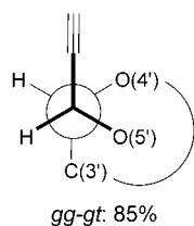
Fig. 2. Calculated population of the conformations obtained by rotation about the C(5')–C(4') bond of \beta -D-ribo-, \beta -D- allylo -hept-6-yno-, and \alpha -L- talo -hept-6-ynofuranosyl-nucleosides
